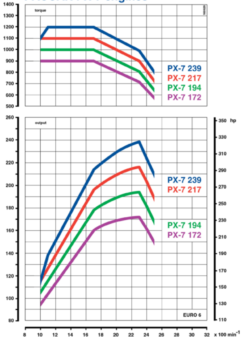
RACCAR PX-7 engines
