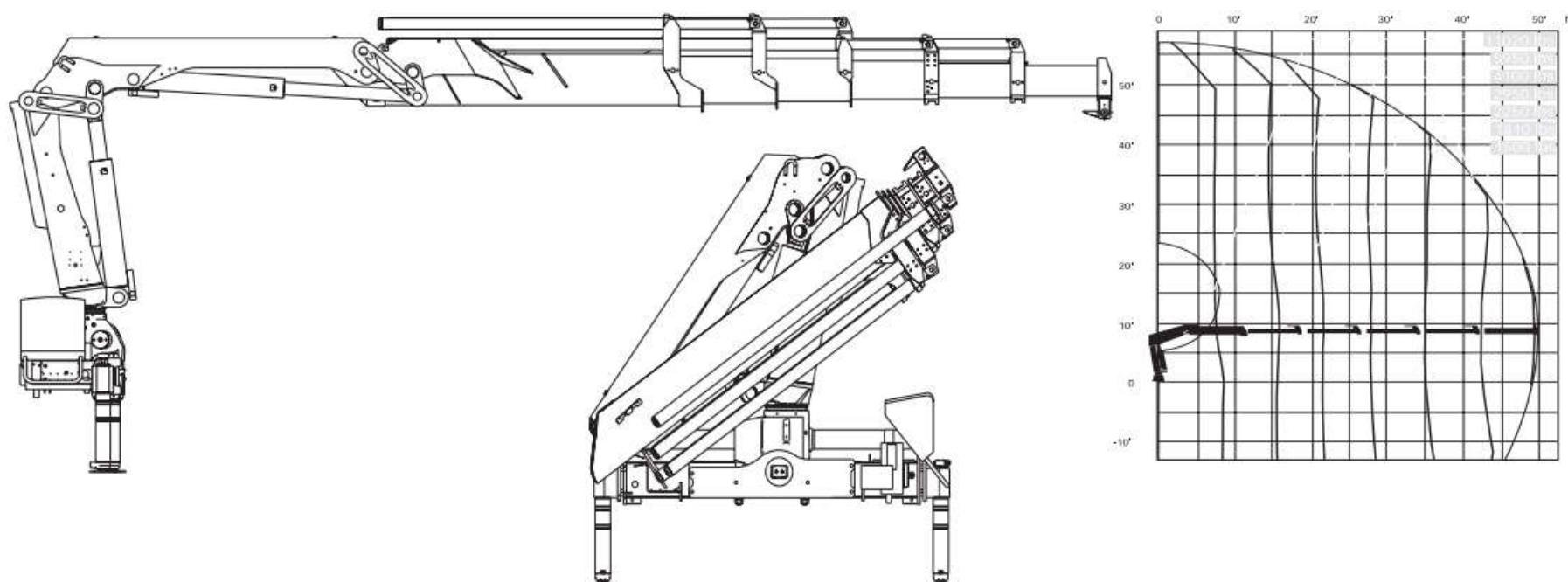
HIAB XS 144 PRO
