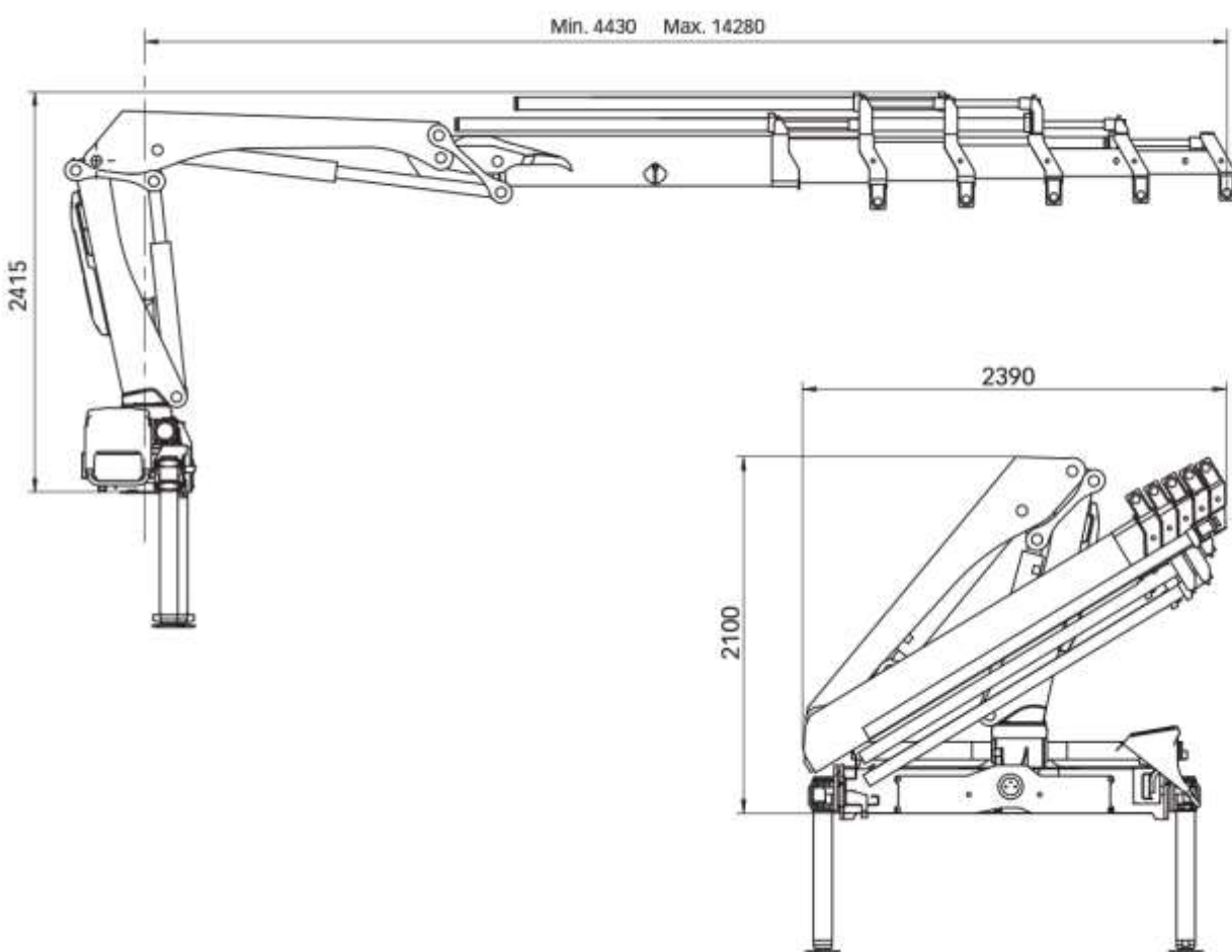
HIAB XS 099 HiDuo
