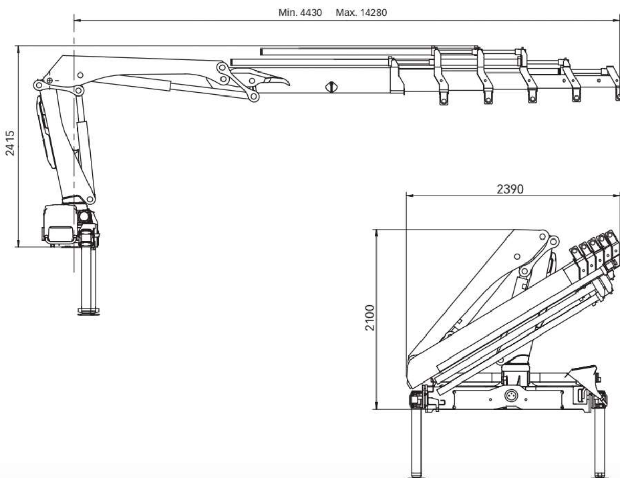
HIAB XS 099 Duo
