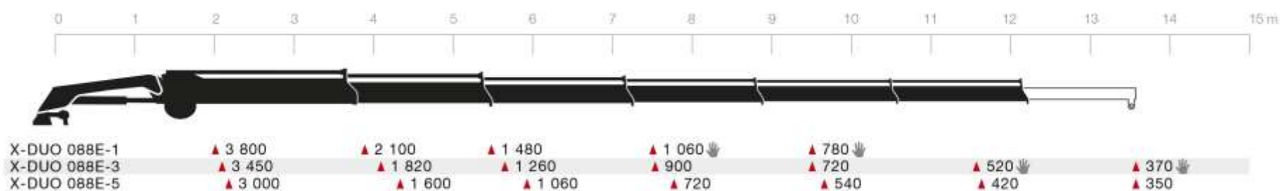
HIAB XS 088 HiPro
