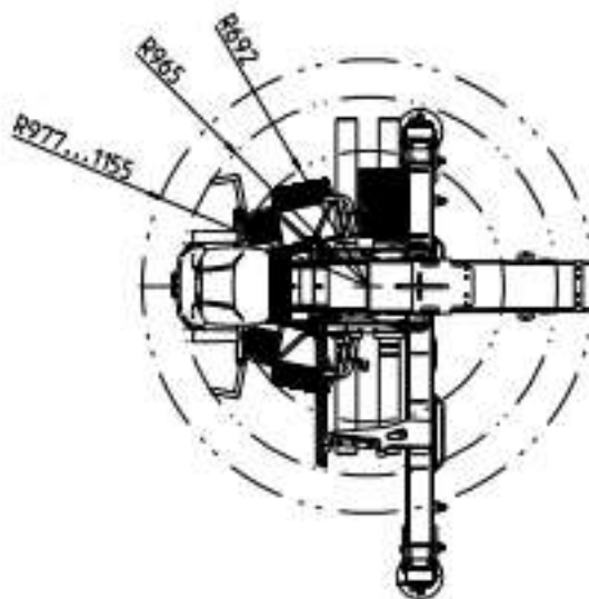
Top view with top seat
