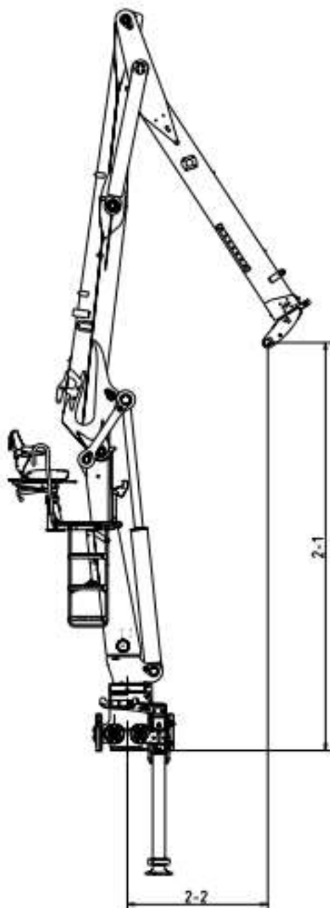
Upright view with top seat
